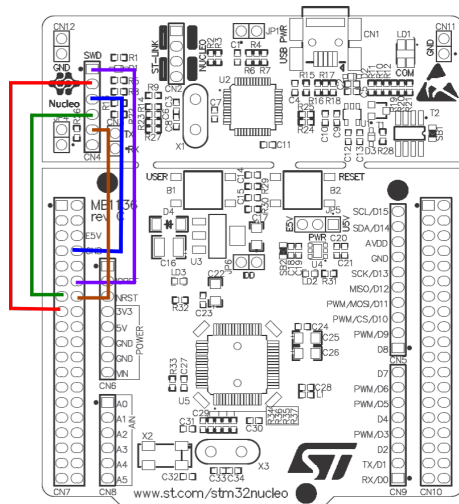
Figure 1: Connection diagram for STLink to cut Nucleo board.
